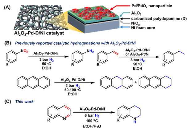
Fig. 1 General schematic for the hierarchical Ni-foam supported Pd catalyst framework (A) previously reported for the catalytic hydrogenation of nitroaromatics, styrenes, and anthracene (B) and the hydrogenation of quinolines (C) reported herein.
