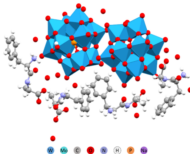
Fig. 7 Molecular structure of the (H 3 O) 2 (HPhe-Ala) 4 [PW 12 O 40 ] 2 \cdot 11H 2 O. 32
