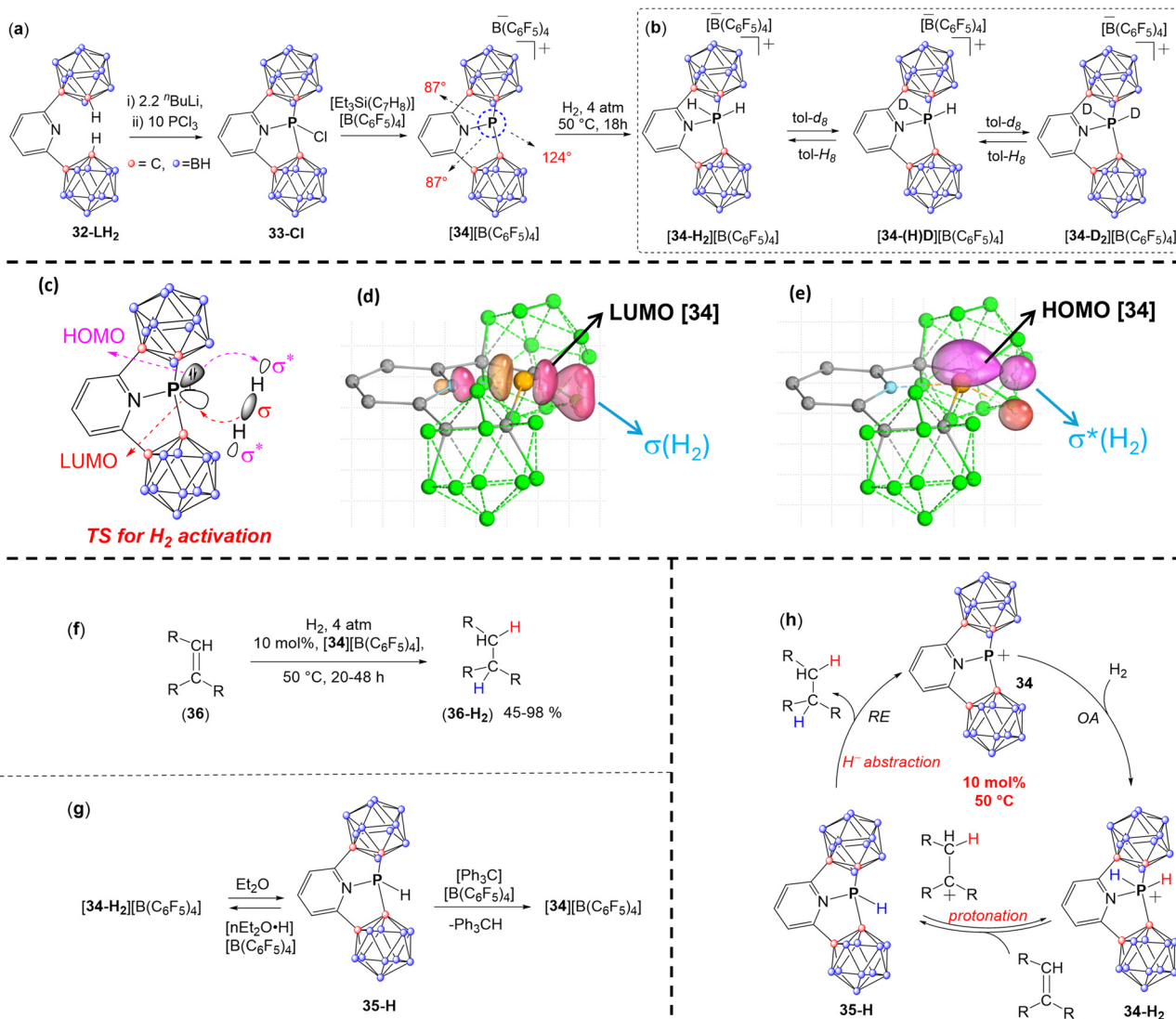
Fig. 13 Synthetic scheme for (a) the synthesis of [\mathbf{34}][\text{B}(\text{C}_6\text{F}_5)_4] ; (b) the activation of dihydrogen by [\mathbf{34}][\text{B}(\text{C}_6\text{F}_5)_4] and toluene- d_8 and vice-versa; (c) schematic representation to show electrophilically driven activation of the H–H bond by \mathbf{34} ; (d) \sigma -bond of \text{H}_2 approaching the P-centre from the direction of the LUMO of \mathbf{34} ; (e) followed by the interaction of the HOMO of the P-centre with the LUMO ( \sigma^* ) of \text{H}_2 ; (f) [\mathbf{34}][\text{B}(\text{C}_6\text{F}_5)_4] catalyzed hydrogenation reactions of unsaturated C–C species; (g) equilibrium of [\mathbf{34}][\text{B}(\text{C}_6\text{F}_5)_4] with \mathbf{35}\text{-H} and reaction of \mathbf{35}\text{-H} with [\text{Ph}_3\text{C}][\text{B}(\text{C}_6\text{F}_5)_4] ; and (h) the proposed catalytic cycle.
