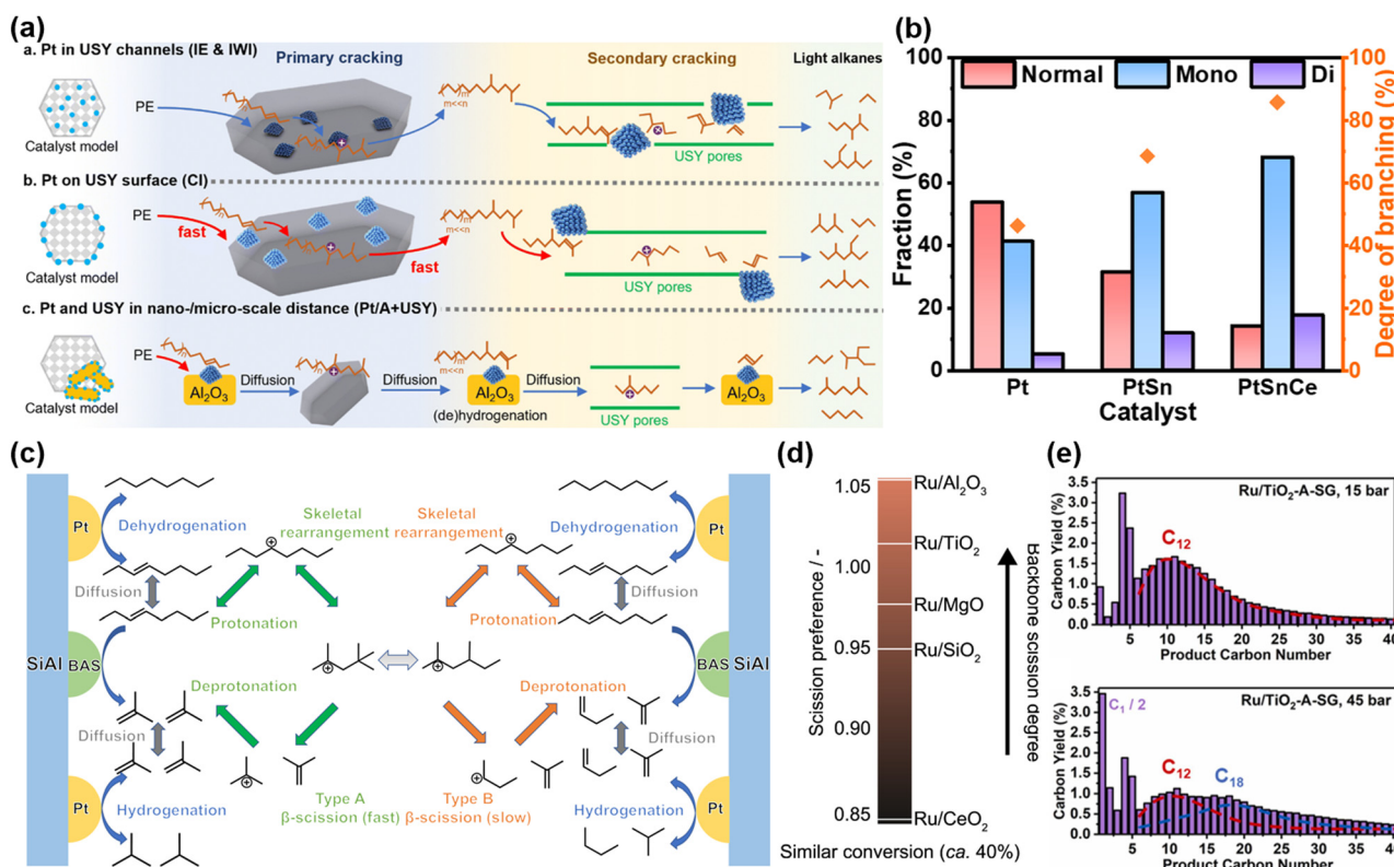
Fig. 2 Recent advances in PO plastic upcycling via hydrogen-assisted processes. (a) Proposed mechanism of hydrocracking of PE on Pt/USY catalysts with varying metal–acid proximities. Reproduced with permission from the Royal Society of Chemistry, copyright 2024. 28 (b) and (c) Investigation of the hydrocracking reaction mechanism. (b) Catalytic tests using n -octadecane as the substrate. (c) Reaction mechanism analysis using n -octane as the reactant model. Reproduced with permission from American Chemical Society, copyright 2023. 30 (d) Scission preferences in PP hydrogenolysis on supports with different basicities. Reproduced with permission from Elsevier, copyright 2023. 34 (e) Product distribution at varying hydrogen pressures. Reproduced with permission from Elsevier, copyright 2023. 35
