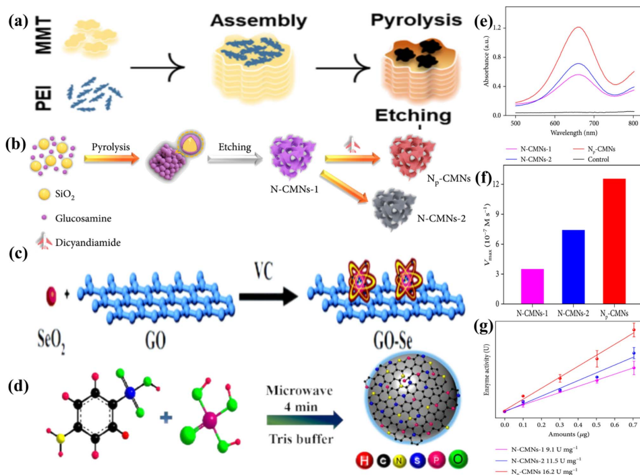
Fig. 3 Synthesis of (a) N-doped carbon sheets via strong electrostatic attraction between MMT and PEI, (b) N-CMNs, (c) GO-Se nano-composites, and (d) NSP-CQDs. (e) UV-vis absorption spectra of POD-like catalytic oxidation with N-CMN-1, \text{N}_p -CMN-2, and Control. (f) V_{\text{max}} ( \text{H}_2\text{O}_2 substrate) and (g) specific activity (SA) of N-CMN-1, N-CMN-2, and \text{N}_p -CMN-2.
