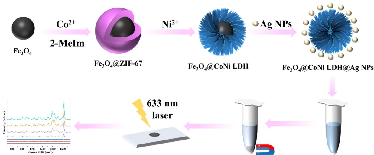
Scheme 1 Schematic of the preparation of the \text{Fe}_3\text{O}_4@\text{CoNi LDH}@\text{Ag NP} SERS substrate and the process used for SERS detection.
