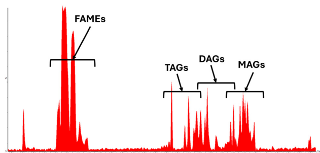
Fig. 10 Base peak ion current chromatogram (BPICCC) of the positive ion ESI SFC-MS for HVO 6.
