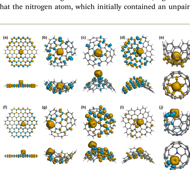
Fig. 7 Spin densities of the Fe(III) complexes in their most stable spin multiplicity configuration: (a) Fe(III)@Planar ( M = 6 ); (b) Fe(III)@Endo ( M = 5 ); (c) Fe(III)@Exo ( M = 5 ); (d) Fe(III)@Negative ( M = 5 ); (e) Fe(III)@Well ( M = 6 ); (f) Fe(III)@N-Planar ( M = 5 ); (g) Fe(III)@N-Endo ( M = 6 ); (h) Fe(III)@N-Exo ( M = 6 ); (i) Fe(III)@N-Negative ( M = 6 ); (j) Fe(III)@N-Well ( M = 5 ). The yellow density represents the excess of \alpha -electron density. The blue density represents the excess of \beta -electron density.
