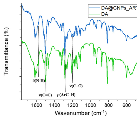
Fig. 8 FT-IR spectra of DA and the DA@CNPs_ART complex.
