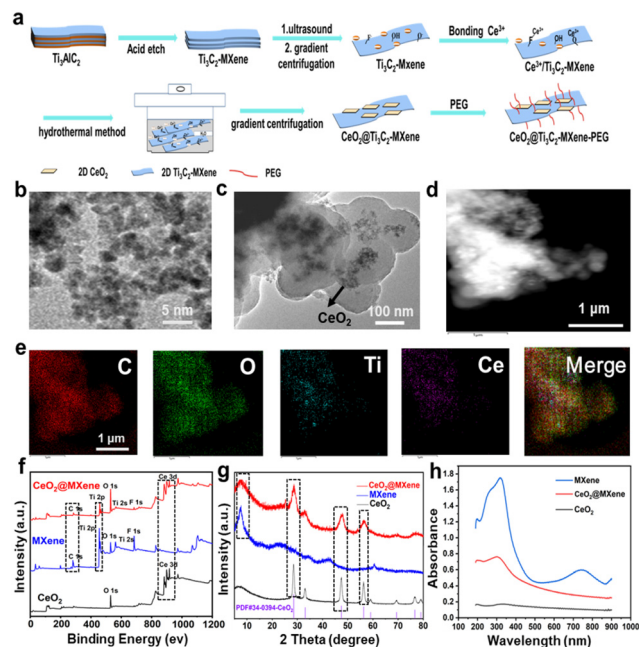
Fig. 1 (a) Schematic diagram of the preparation of the \text{CeO}_2@MXene heterojunction. (b) TEM image of \text{CeO}_2 . (c) TEM image of \text{CeO}_2@MXene . (d) and (e) \text{CeO}_2@MXene -STEM images and the corresponding elemental mapping images for C, O, Ti, and Ce. (f) X-ray photoelectron spectroscopy images of \text{CeO}_2/\text{MXene}/\text{CeO}_2@MXene . (g) XRD pattern of \text{CeO}_2/\text{MXene}/\text{CeO}_2@MXene . (h) Absorption spectra of \text{CeO}_2/\text{MXene}/\text{CeO}_2@MXene .
