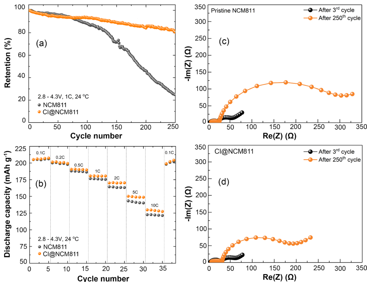
Fig. 8 (a) Cycle retention at room temperature and (b) rate capability of pristine NCM811 and CI@NCM811 in the half-cell test. The Nyquist plots of (c) pristine NCM811 and (d) CI@NCM811.
