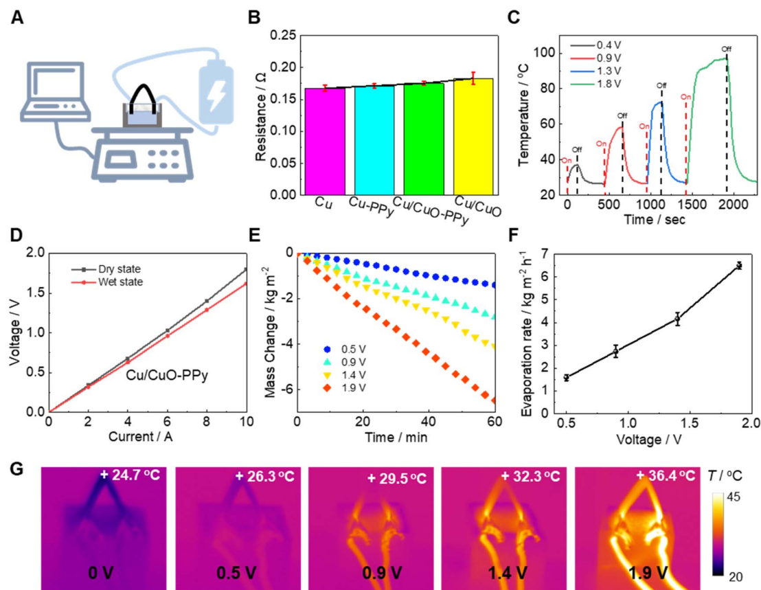
Fig. 3 Night time evaporation performance via Joule heating. (A) Schematic illustration of the evaporation driven by Joule heating; (B) electrical resistance of dried Cu, Cu-PPy, Cu/CuO, and Cu/CuO-PPy foams; (C) temperature changes of dried Cu/CuO-PPy foam (20 mm \times 20 mm \times 1 mm) subjected to different voltages; (D) CV curves of the Cu/CuO-PPy foam under dried and wet conditions; (E) mass changes and (F) evaporation rates of the dual-side 3D evaporator driven by Joule-heating at different voltages; (G) steady-state temperature of the dual-side 3D Cu/CuO-PPy evaporator subjected to different voltages.
