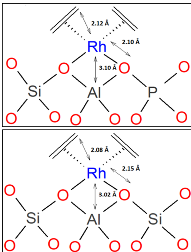
Scheme 1 Structural models of rhodium diethene complex on SAPO-37 (top) 61 and rhodium diethene complex on DAY zeolite (bottom) 60 determined by EXAFS spectroscopy. Reproduced from ref. 61 with permission from the American Chemical Society, Copyright 2021.
