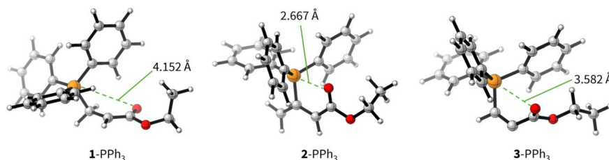
Fig. 11 Molecular structures of the zwitterionic adducts of \text{PPh}_3 with 1 , 2 , and 3 optimised at SMD(DCM)/MN15/def2-TZVPP level of theory. Green dashed lines indicate relevant P–O distances in the adducts.
