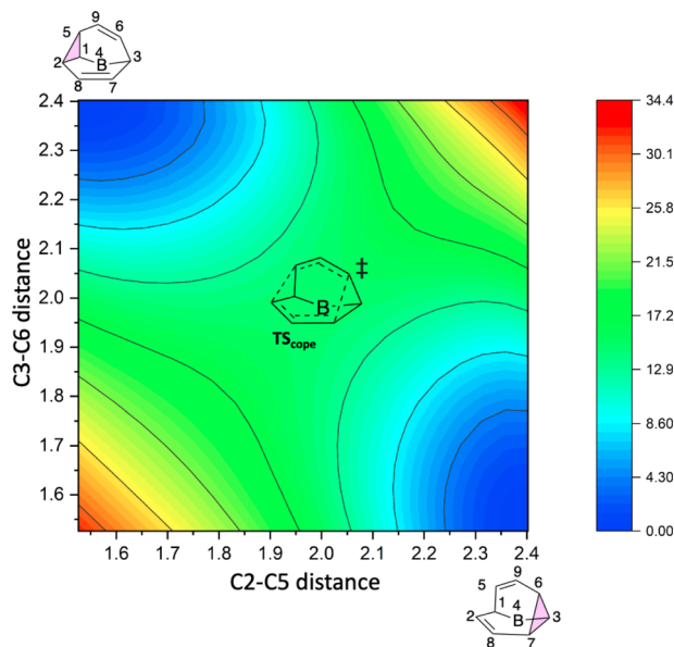
Fig. 10 2D potential energy surface for [3s,3s] sigmatropic shift of B_{C_8}H_9 .
