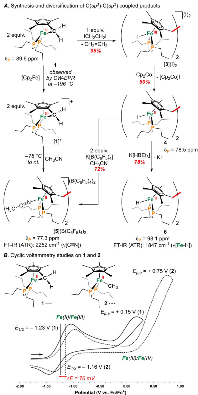
Fig. 2 (A) Synthesis of [1]^+ and \text{C}(\text{sp}^3)\text{-C}(\text{sp}^3) coupled products. (B) Cyclic voltammograms for 1 and 2 .
