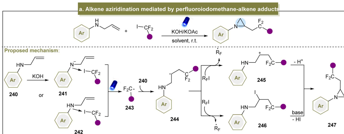
Scheme 11 (a) Alkene aziridination mediated by a perfluoriodomethane–alkene adduct.
