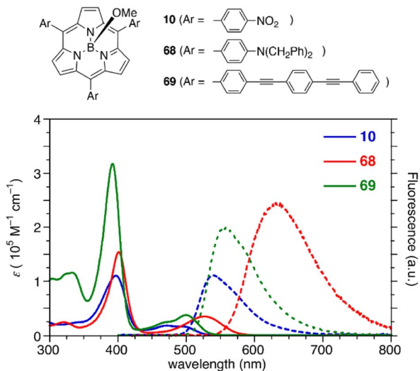
Fig. 5 UV-vis absorption (solid line) and fluorescence (dashed line) spectra of subporphyrins 10 , 68 , and 69 bearing 4-substituted phenyl groups at the meso -positions in CH 2 Cl 2 .
