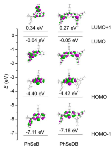
Fig. 4 Molecular orbital patterns (isocontour value = 0.025) for PhSeB and PhSeDB based on their optimized S 0 geometries.
