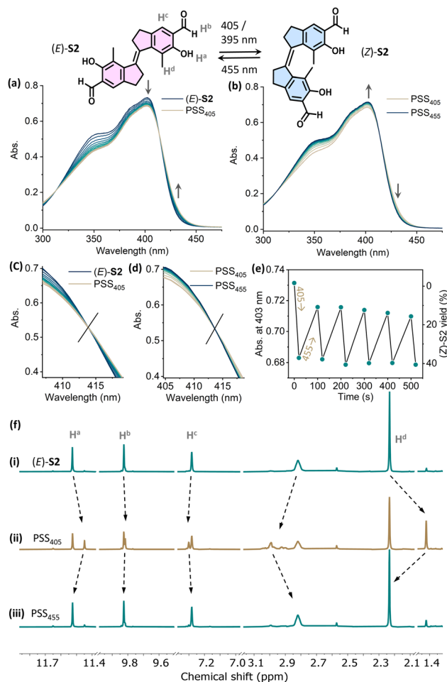
Fig. 4 Changes in the UV-vis absorption spectra starting from (a) (E)-S2 (24 μM in CH 2 Cl 2 , 298 K) upon irradiation with 405 nm light to PSS 405 and (b) upon subsequent irradiating with 455 nm light to PSS 455 . Enlarged spectra at the isosbestic point of (c) E to Z isomerization and (d) Z to E back-switching. (e) Plots of the absorption at λ = 403 nm upon sequential irradiation with 405 nm and 455 nm light. (f) Changes in 1 H NMR spectra of (i) (E)-S2 (2.9 mM in CD 2 Cl 2 , 298 K, 500 MHz), (ii) upon irradiation with 405 nm light to PSS 405 , and (iii) upon subsequent irradiation with 455 nm light to PSS 455 .
