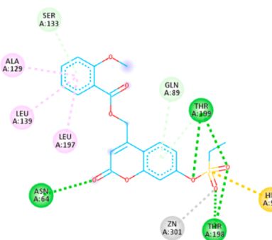
Fig. 124 Chemical structures of compounds 348–352; their IC_{50} values against hCA-II, IX and XII along with their docking images.
