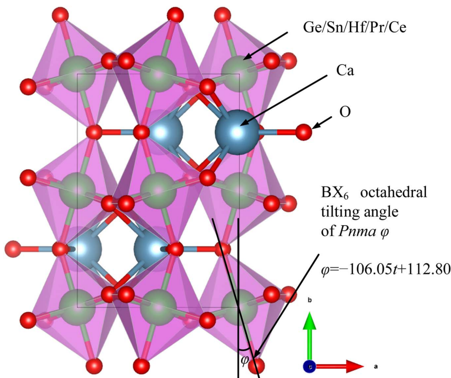
Fig. 2 The relationship between BX 6 octahedral tilting angle and crystal structure.
