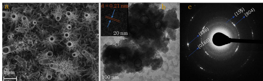
Fig. 1 (a) SEM image, (b) TEM image (inserted HRTEM), and (c) SAED of \text{Cu}_7\text{S}_4 at 96 h.
