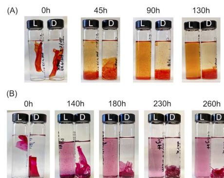
Fig. 3 Stages of light disassembly of multilayer film (A) CS–ALR (mass ratio 1/0.125) in 1% acetic acid solution (pH = 3) at 20 °C under 460 nm blue light irradiation. (B) CS–AMA (mass ratio 1/0.125) in 1% acetic acid solution at 20 °C under 520 nm green light irradiation. For all photographs: samples “L” were exposed to light and control samples “D” were in the dark.
