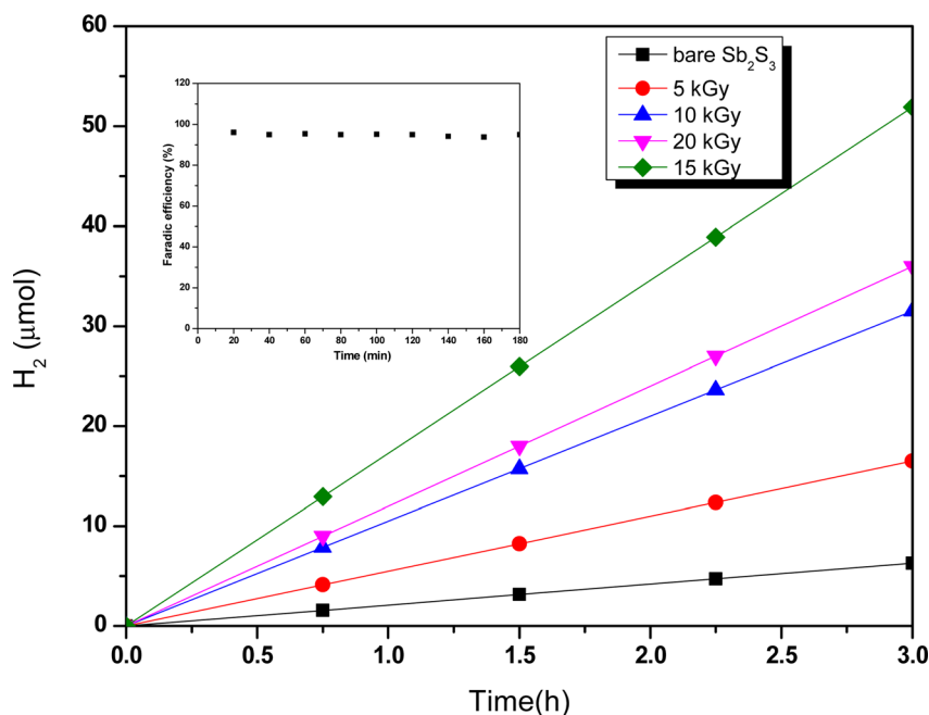
Fig. 18 Hydrogen evolution as a function of time for different Sb 2 S 3 -based photocathodes under standard one sun (100 mW cm -2 ) illumination at 0 V vs. RHE. The inset plot of Fig. 15 stands for the faradaic efficiency (FE) measurement of the optimized Sb 2 S 3 -based photocathode (15 kGy).
