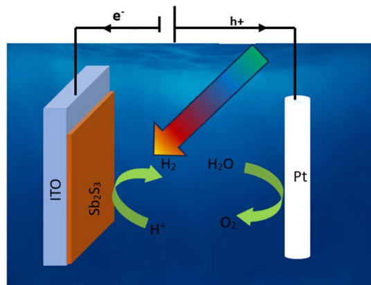
Fig. 17 Schematic mechanism of photoelectrochemical water splitting of Sb 2 S 3 -based photocathode.
