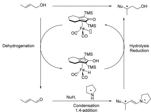
Scheme 74 Dual iron/organocatalysed alkylation of allylic alcohols.
