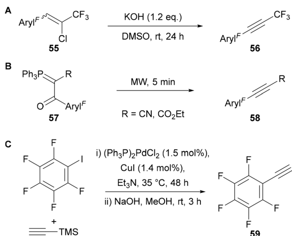
Scheme 20 Preparation of polyfluoroaryl-alkynes. \text{Aryl}^{\text{F}} = polyfluoroaryl.
