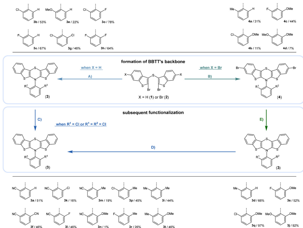
Scheme 1 Modular synthesis of sterically restricted BBTTs 3 yielding a functionalization with electron accepting to electron donating substituents in the ortho or ortho,ortho' -position of the N -aryl moiety: (A) ortho ( ortho' )-disubstituted aniline (1.00 equiv.), Pd(dba) 2 (5.00–7.50 mol%), DPPF or XantPhos (10.0–15.0 mol%), NaO t Bu (3.00 equiv.), 110 °C in toluene; (B) ortho ( ortho' )-aniline (1.00 equiv.), Pd(dba) 2 (3.00–5.00 mol%), BINAP (5.00–10.0 mol%), NaO t Bu (3.00 equiv.), 110 °C in toluene; (C) MeMgCl (1.20–2.40 equiv.), PEPPSI-IPr (10.0–15.0 mol%), 60 °C in THF; (D) K 4 [Fe(CN) 6 ]·3H 2 O (0.250–5.00 equiv.), PEPPSI-IPr (5.00–20.0 mol%), Na 2 CO 3 (2.50–5.00 equiv.), 160 °C in DMF; (E) (I) t BuLi (2.40 equiv.), TMEDA (2.40 equiv.), –78 °C in THF and (II) methanol (10.0 equiv.), –78–22 °C in THF.
