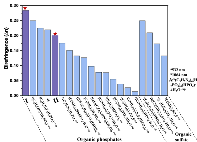
Fig. 7 Birefringence comparison between title compounds and reported phosphates or sulfates containing organic groups.
