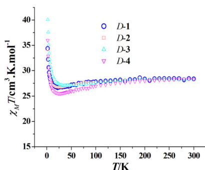
Fig. 5 Plots of \chi_{\text{M}}T versus T of D-1 , D-2 , D-3 and D-4 ( H_{\text{dc}} = 1000 \text{ Oe} ).
