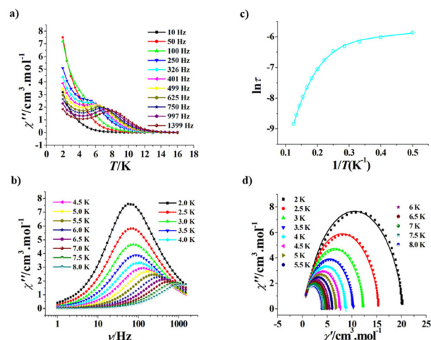
Fig. 6 Plots of \chi'' versus T for D-1 ( H_{\text{dc}} = 0 \text{ Oe} ) (a). Frequency dependence of \chi'' for D-1 at a zero dc field (b). Plot of \ln \tau versus 1/T for D-1 ( H_{\text{dc}} = 0 \text{ Oe} ); the solid line represents the best fitting with quantum tunnelling plus Orbach plus Raman (c). Cole–Cole plots measured from 2.0 to 8.0 K for D-1 ( H_{\text{dc}} = 0 \text{ Oe} ); the solid lines represent the best fitting with the generalized Debye model (d).
