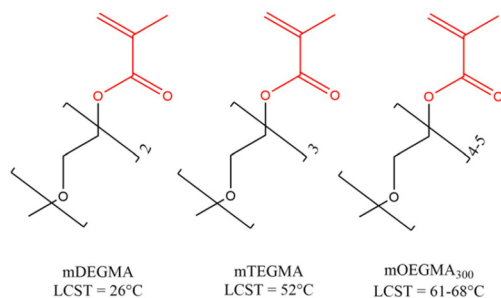
Fig. 8 Non-linear PEG derivatives and their LCST. 94 mDEGMA – di(ethylene glycol) methyl ether methacrylate; mTEGMA – tri(ethylene glycol) methacrylate; mOEGMA – oligo(ethylene glycol) methyl ether methacrylate.
