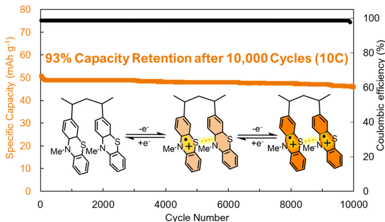
Fig. 4 Cycling performance of poly(3-vinyl-N-methylphenothiazine) at a 10C rate. Structure depicted visualizes the \pi - \pi interactions between the monomer units during different stages of charge/discharge. Adapted with permissions from ref. 35. Copyright © 2017 Royal Society of Chemistry.
