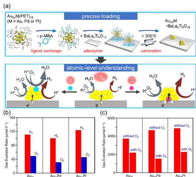
Fig. 5 (a) Schematic illustration of the synthesis procedure for the \text{Au}_{24}\text{M}/\text{BaLa}_4\text{Ti}_4\text{O}_{15} photocatalyst ( \text{M} = \text{Au, Pd, or Pt} ) and the role of the dopant in the HER. (b) Hydrogen and oxygen evolution rates for \text{Au}_{25} , \text{Au}_{24}\text{Pd} and \text{Au}_{24}\text{Pt} in photocatalytic water splitting under UV light. (c) Difference in the hydrogen evolution rate in the presence of methanol as a sacrificial reagent under a flow of Ar gas (without \text{O}_2 ) and a 7:3 mixture ratio of Ar to air (with \text{O}_2 ). Reproduced from ref. 49 with permission from the American Chemical Society, Copyright 2019.
