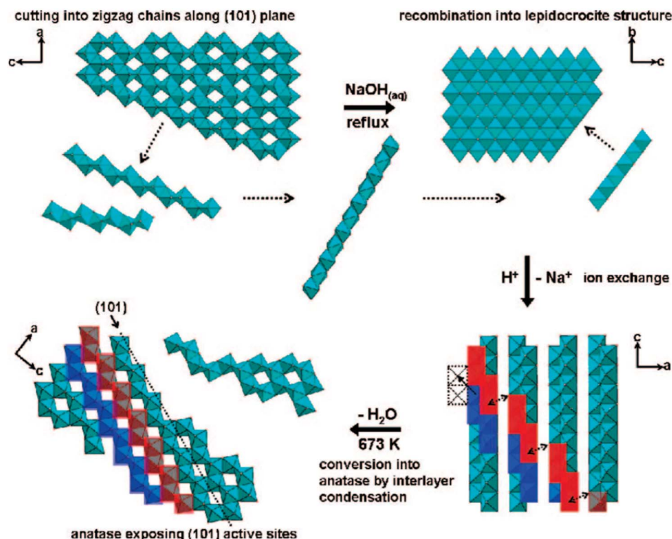
Fig. 2 Schematic illustration of the conversion pathway of commercial bulk anatase to two-dimensional (101)-exposed anatase \text{TiO}_2 nanosheet in the chimie-douce method. Reprinted with permission from ref. 48. Copyright 2008, American Chemical Society.
