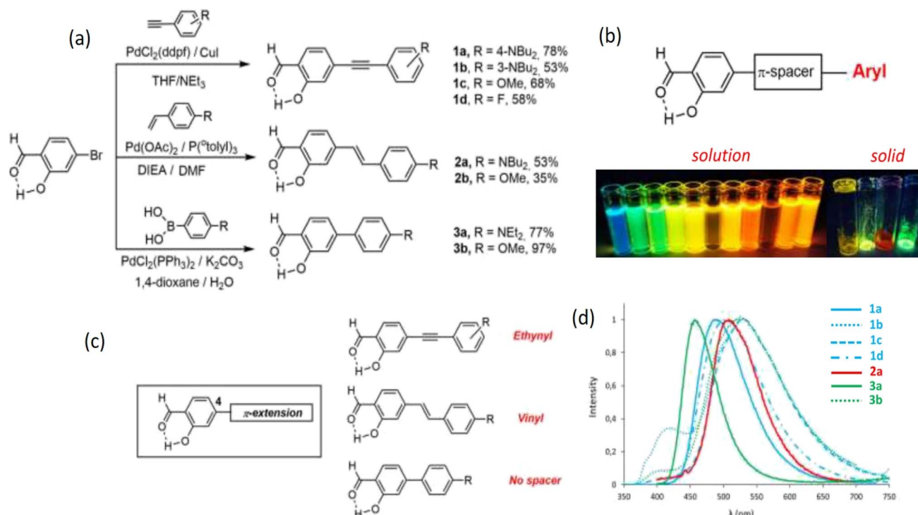
Fig. 1 (a) Synthesis protocol of 4-extended SD derivatives 1a–d , 2a–b , and 3a–b . (b) Compounds of SD that exhibit intense fluorescence in multiple environments in solution and solid state. (c) 4-Extended SD derivatives. (d) SD's emission spectra in aerated solutions of toluene at room temperature are as follows: 1a (plain blue), 1b (dotted blue), 1c (dashed blue), 1d (dotted dashed blue), 2a (plain red), 2b (dotted red), 3a (plain green), and 3b (dotted green). Reproduced with permission from ref. 22, copyright 2024, Eur. J. Org. Chem.
