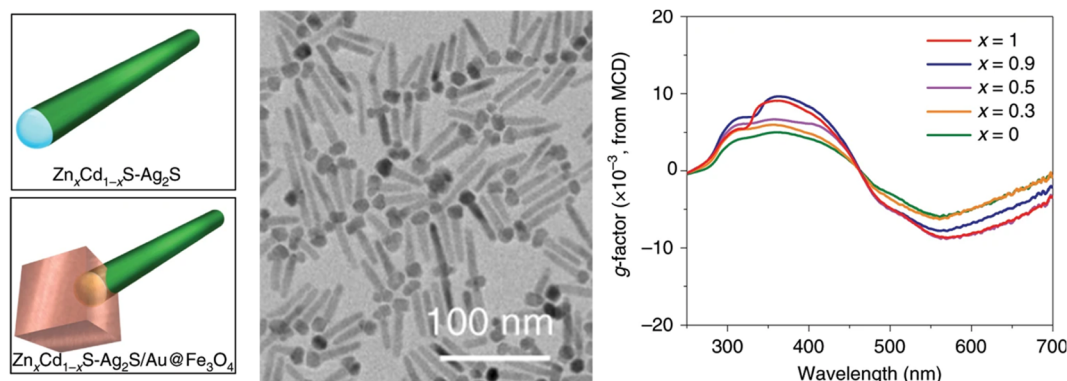
Fig. 9 Multicomponent hybrid materials with magnetically induced chirality. Geometric models, TEM image, and magnetic CD spectra of Zn_xCd_{1-x}S-Ag_2S/Au@Fe_3O_4 hybrid materials. 70 Reproduced from ref. 70 with permission from Springer Nature, copyright 2020.
