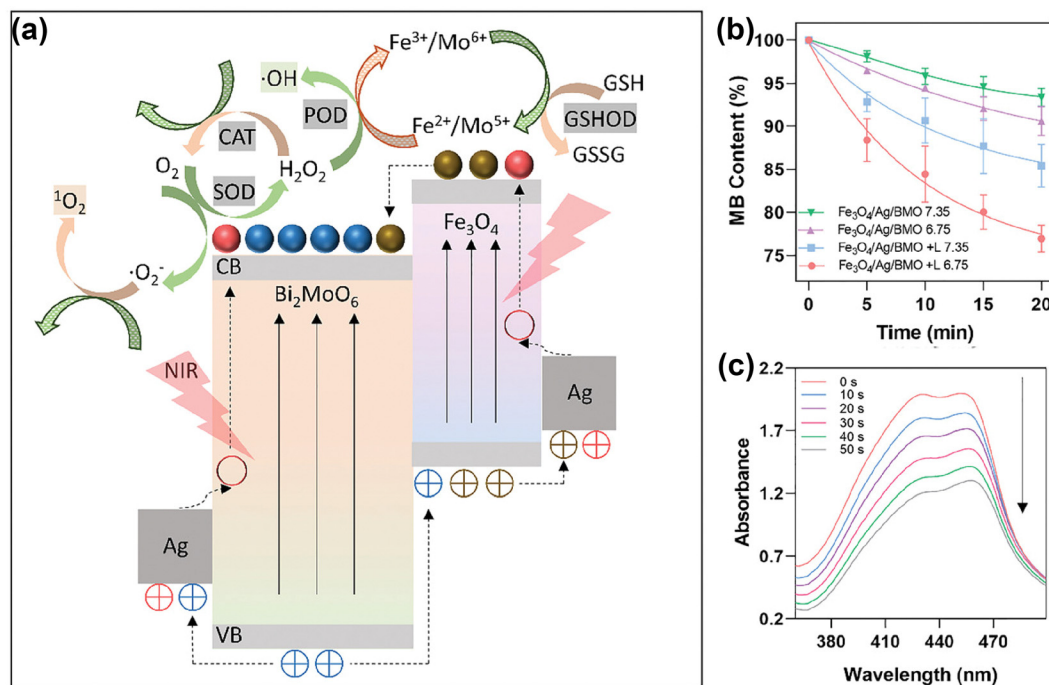
Fig. 6 (a) Schematic illustration of the working mechanisms underlying the intraparticle interactions of BMO NP. (b) Degradation of MB for •OH generation. (c) Light adsorption of DPBF decreases due to 1 O 2 generation under laser irradiation with different durations (0–50 s). Reproduced with permission from ref. 53. Copyright 2021, Wiley.
