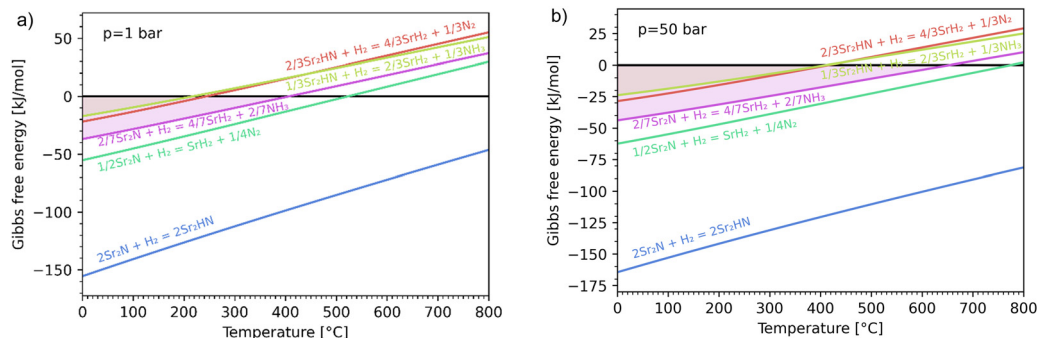
Fig. 4 Ellingham diagram of the hydrogenation step for the reactions (7)–(11). Variation of the Gibbs free energy change per mol H 2 as a function of temperature for: (a) standard \Delta G_{rxn}^\circ ; and (b) \Delta G_{rxn} at 50 bar assuming 20% reaction extent.
