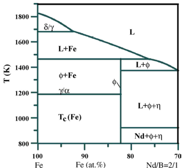
Fig. 9 Schematic representation of the quasi-binary phase diagram of the Nd-Fe-B system, highlighting the crucial phase formations near the peritectic point. 32
