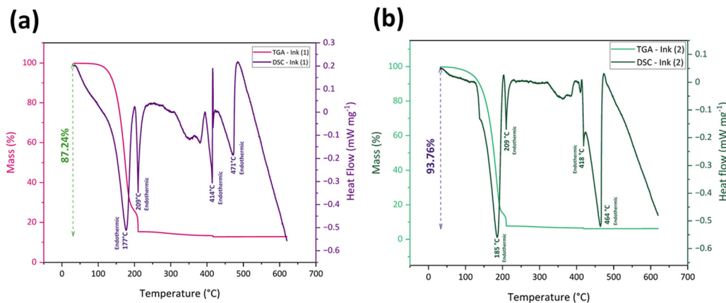
Fig. 4 TGA/DSC curves of (a) Ink (1) and (b) Ink (2).
