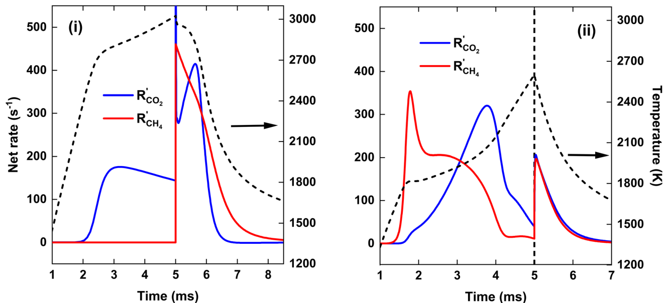
Fig. 8 Net rates of conversion of \text{CO}_2 and \text{CH}_4 , as a function of time, for SEI = 140 \text{ kJ mol}^{-1} (left y-axis). The temperature is indicated by the dashed black line (right y-axis). The left panel (i) and right panel (ii) show the results for the \text{CO}_2 plasma with post-plasma \text{CH}_4 injection, and for the \text{CO}_2/\text{CH}_4 plasma with post-plasma \text{CO}_2/\text{CH}_4 injection, respectively.
