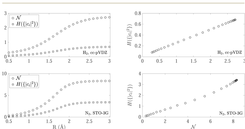
Fig. 7 Nonfreeness \mathcal{N} and Shannon entropy H(\{|c_i|^{(B)}|^2\}) of the CI expansion coefficients in natural orbital basis for the full CI ground state of \text{N}_2 in the STO-3G basis at various internuclear distances R (left), and H(\{|c_i|^{(B)}|^2\}) as a function of \mathcal{N} (right).
