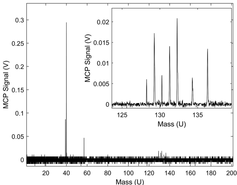
Fig. 1 Typical TOF-MS trace observed from the reaction of Xe^+ with C_3H_4 . Primary plot displays the trace's full signal intensity. Peaks observed in the primary plot, from left to right, correspond to 39 m/z ( c-C_3H_3^+ , product), 40 m/z ( Ca^+ ), 57 m/z ( CaOH^+ ), 128–136 m/z ( Xe^+ ). Inset displays the Xe^+ signals when viewed with greater voltage resolution.
