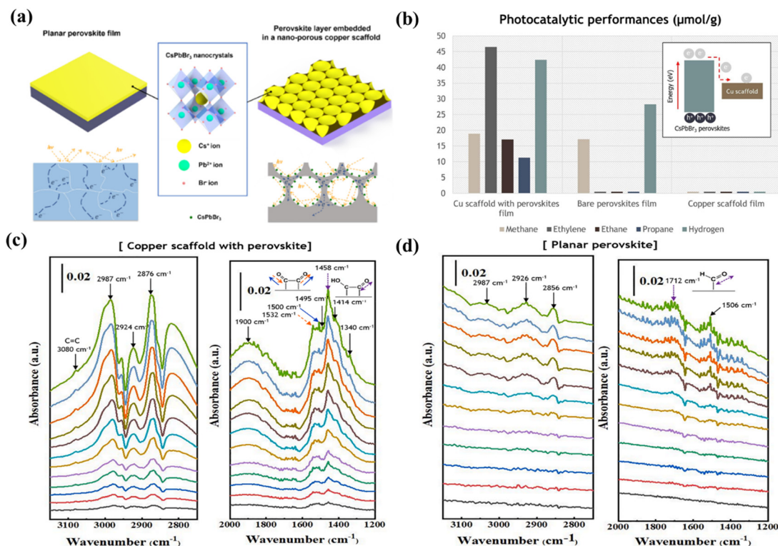
Fig. 19 (a) Comparison of the charge transport processes in a planar perovskite film and the perovskite layer embedded in a nanoporous copper scaffold. 141 (b) Yield of the \text{CO}_2 reduction products after 5 h of photochemical reaction. The inset image represents the relative energetic diagram of the \text{CsPbBr}_3 perovskites within a porous copper scaffold, which acts as an assistant for electron transfer in photocatalytic \text{CO}_2 reduction. 141 (c) In situ ATR-IR spectra of photocatalytic \text{CO}_2 reduction on the \text{CsPbBr}_3 perovskite photocatalyst embedded in a porous copper scaffold. 141 (d) In situ ATR-IR spectra of photocatalytic \text{CO}_2 reduction on the \text{CsPbBr}_3 perovskite photocatalyst embedded in a porous copper scaffold. 141
