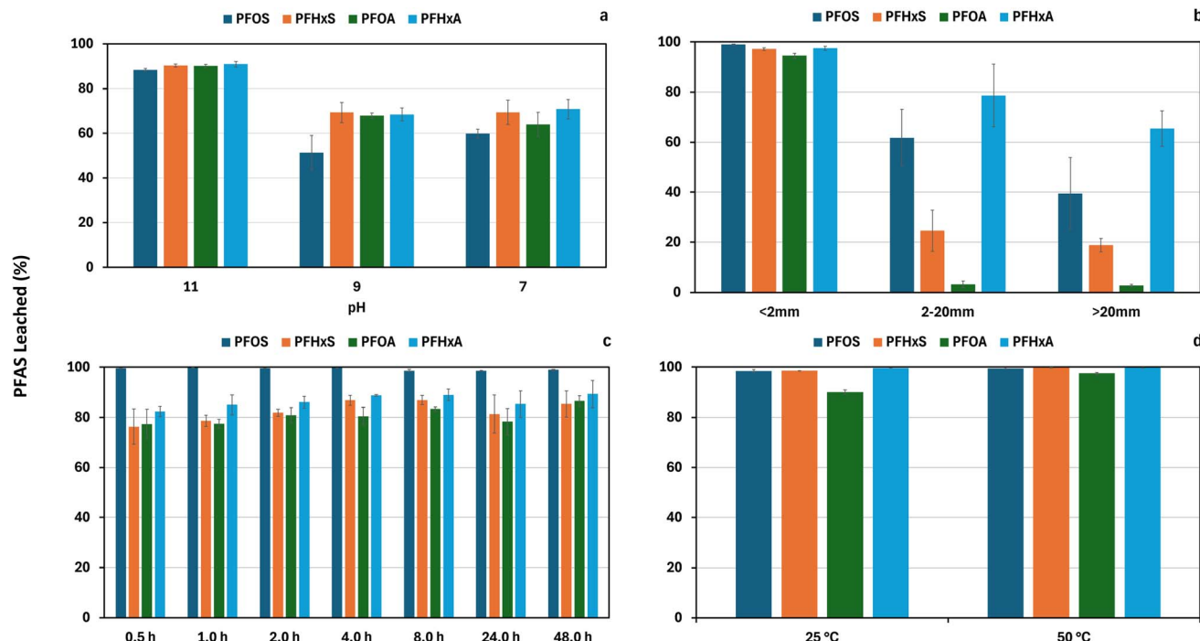
Fig. 6 Effect of (a) pH, (b) particle size, (c) duration of exposure to water and (d) temperature on PFAS leachability from concrete powder.
