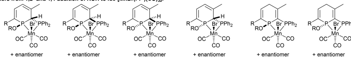
Fig. 1 Selected isomers generated from reactions of 2-phosphinophosphinine (PP') complexes.
