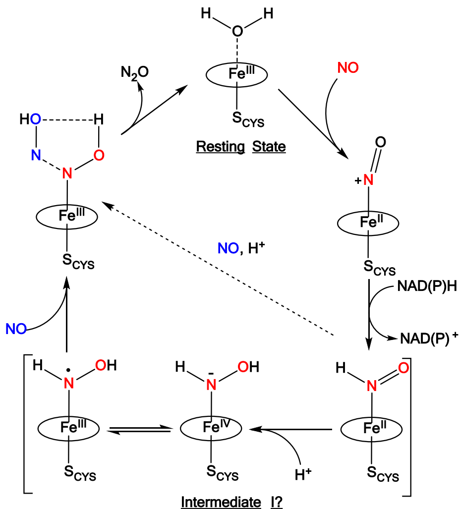
Scheme 1. Proposed mechanism for \text{N}_2\text{O} formation in Cyt. P450nor. The oval represents a generic porphyrin ligand. Reproduced with permission from ref. 1 . Copyright 2021 American Chemical Society.
