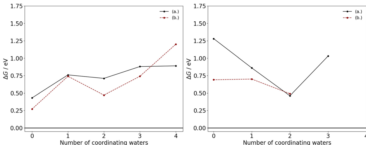
Fig. 3 \Delta G as a function of the number of coordinating water ligands in the neutral molecular complexes of Mn(II) (left) and Mn(III) (right), with acetate ligands in their monodentate coordination mode. In each graph, the competing mechanisms of eqn (4) and (5) are considered as replacement of the acetate species by (a.) acetic acid or (b.) water.
