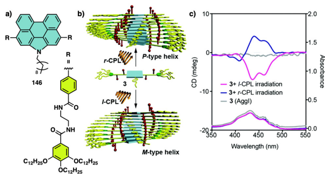
Fig. 69 (a) Structure of 146 . (b) Schematic illustration of the asymmetry induction by CP-light irradiation. (c) ECD Spectra of the opposite handed helical structures generated by irradiation with CP-light. Reproduced from ref. 120 with permission from the Royal Society of Chemistry, copyright 2020.
