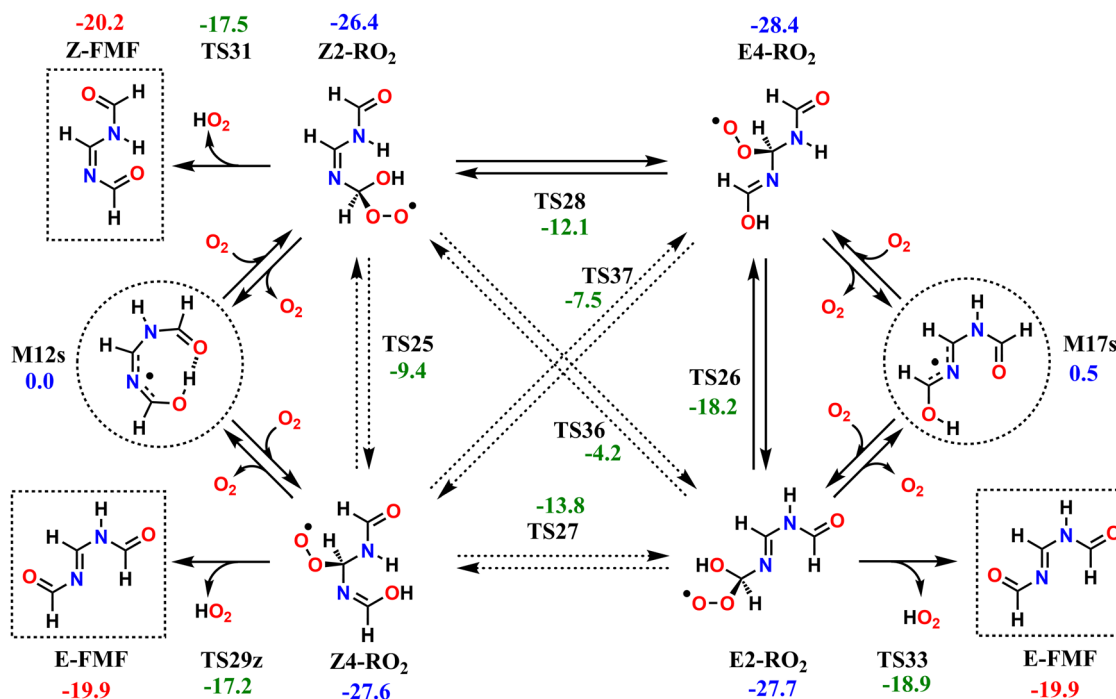
Scheme 2 Studied reaction pathways available to the second-generation RO 2 from imidazole + OH reaction, beginning with M12s and M17s, circled. Relative zero-point-corrected energies given in kcal mol -1 , calculated at the ROHF-ROCCSD(T)-F12a/cc-pVDZ-F12//ωB97X-D/aug-cc-pVTZ level of theory. Major products are shown in dashed squares.
